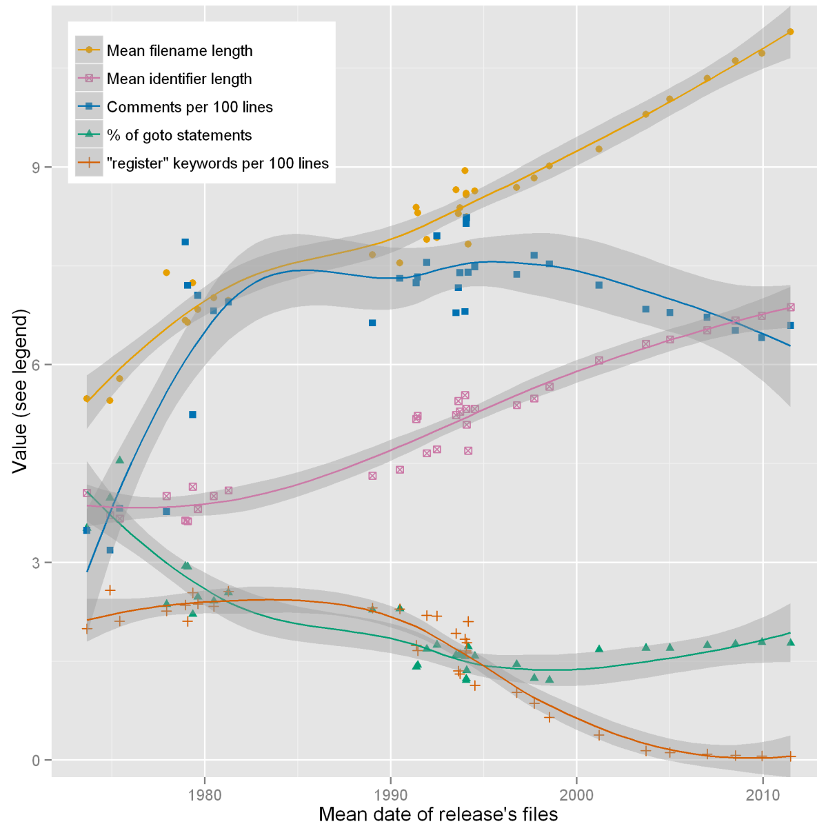
Figure 12: Code style evolution along Unix releases.
