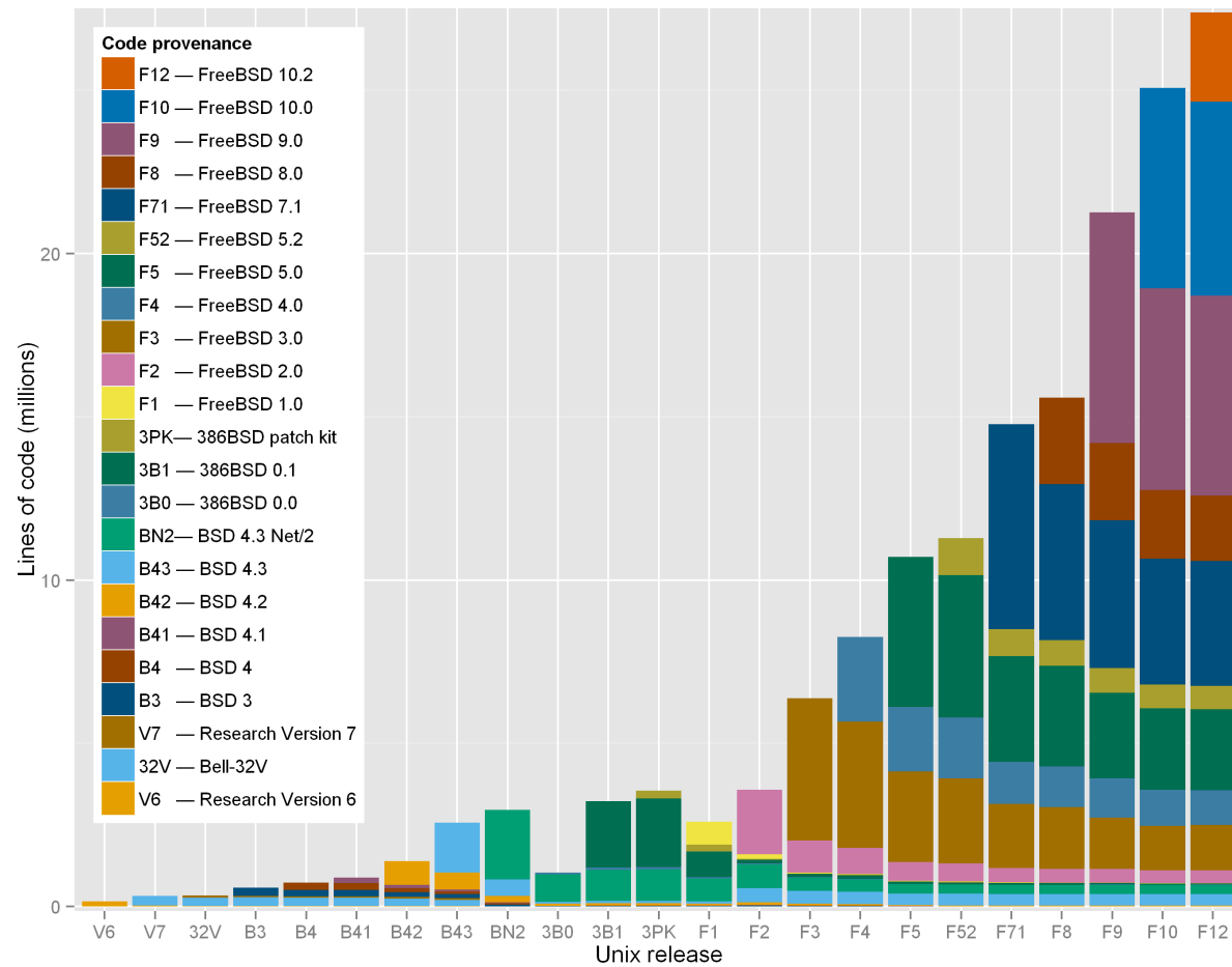
Figure 5: Code growth and provenance across representative Unix releases.
