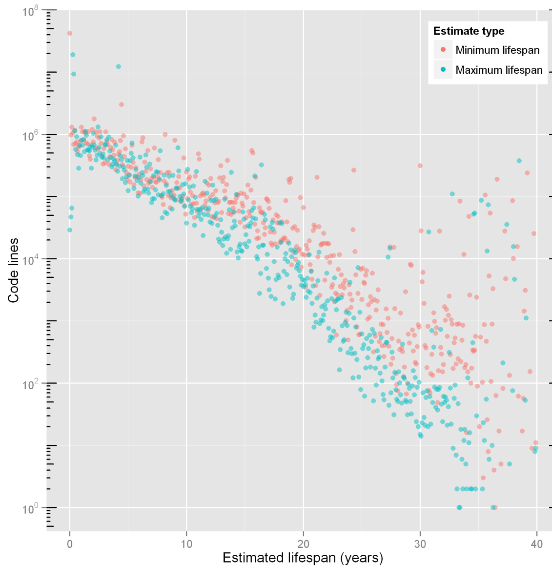
Figure 13: Exponential decay of Unix source code.
